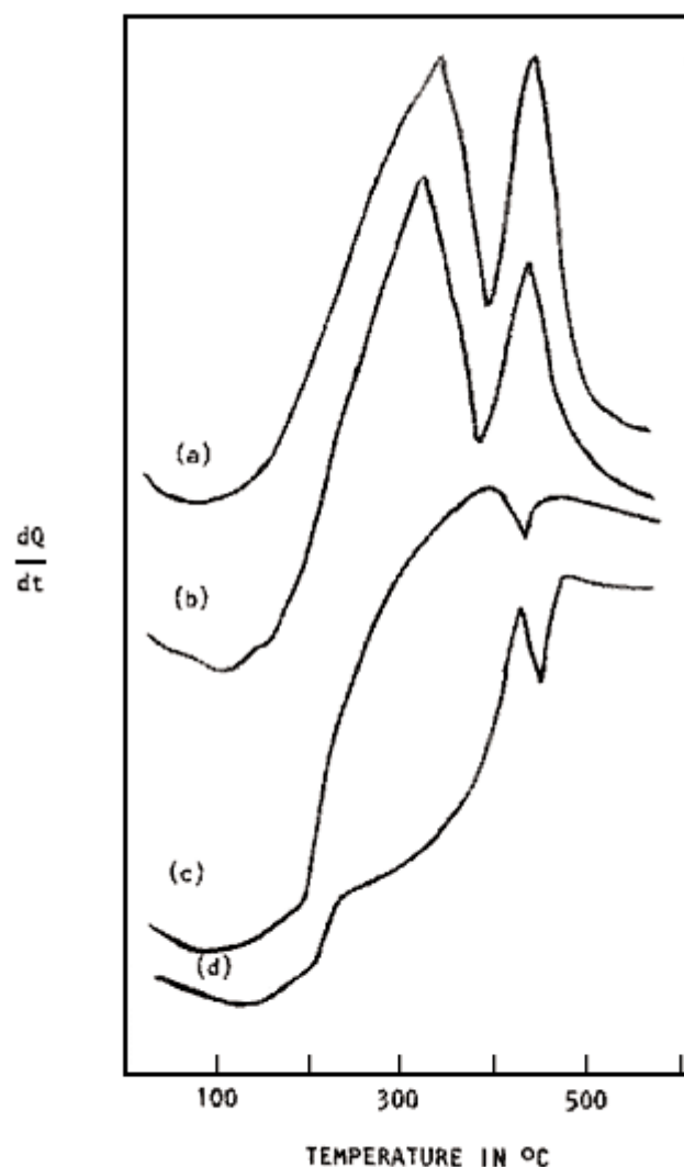
FIGURE 2 - DSC curves of the compounds: (a) \text{Mg}(\text{DMCP})_2 \cdot \text{H}_2\text{O} ; (b) \text{Ca}(\text{DMCP})_2 \cdot 2.5\text{H}_2\text{O} ; (c) \text{Sr}(\text{DMCP})_3 \cdot \text{H}_2\text{O} and (d) \text{Ba}(\text{DMCP})_2 \cdot \text{H}_2\text{O} .
