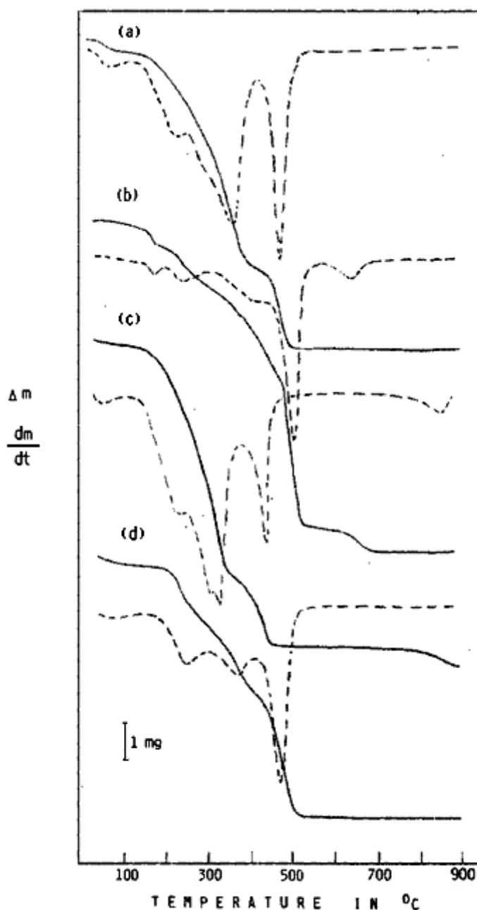
FIGURE 1 - TG and DTG curves of the compounds: (a) \text{Mg}(\text{DMCP})_2 \cdot \text{H}_2\text{O} (6.962); (b) \text{Ca}(\text{DMCP})_2 \cdot 2.5\text{H}_2\text{O} (7.658 mg); (c) \text{Sr}(\text{DMCP})_2 \cdot \text{H}_2\text{O} (7.734 mg) and (d) \text{Ba}(\text{DMCP})_2 \cdot \text{H}_2\text{O} (7.664 mg).
