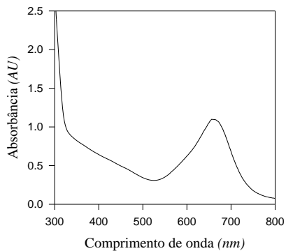
Figura 5. Espectro visível do complexo dimérico [(\text{H}_2\text{O})(\text{L})_2\text{Ru}-\text{O}-\text{Ru}(\text{L})_2(\text{OH}_2)](\text{PF}_6)_4 ( 0,10 \text{ mmol L}^{-1} ) em \text{CH}_2\text{Cl}_2 .
