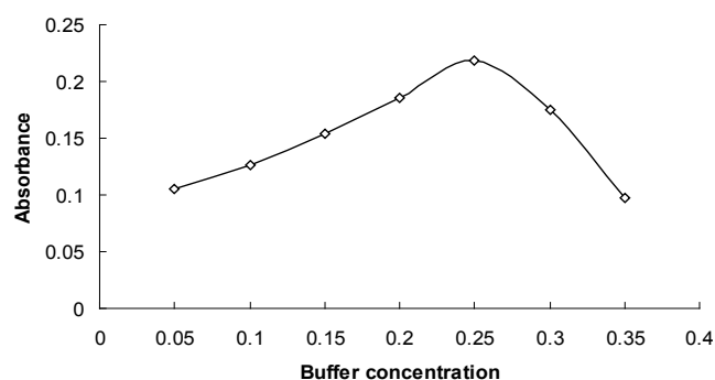
Figure 2: The effect of buffer concentration on the absorbance of U(VI)-EBT complex in the presence of cationic surfactant CTAB at 637 nm.
