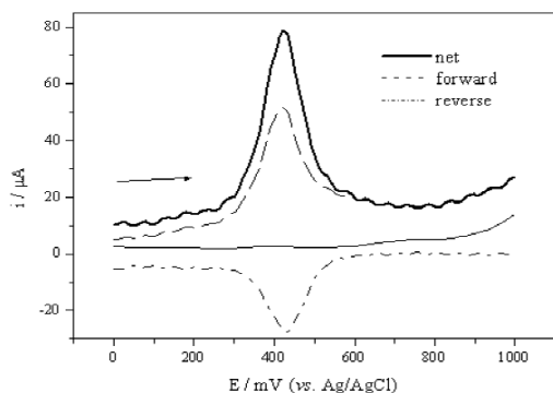
Figure 1. Voltammograms of SWV obtained for 60% (graphite, w/w) composite electrode using 5.0 \cdot 10^{-5} mol L -1 HQ in acetate buffer pH 4.5, f = 50 s -1 , \Delta E_p = 50 mV, \Delta E_s = 10 mV.
