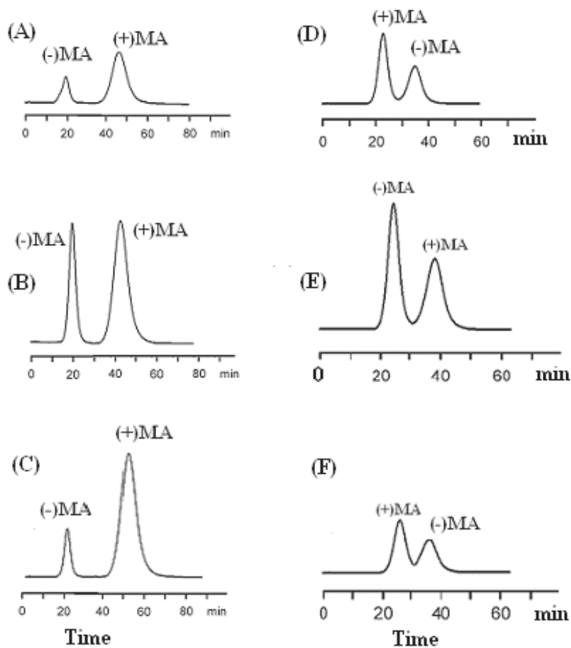
Figure 6: Separation of enantiomers of mandelic acid using MIP with (+)-mandelic acid as template (A-C), (-)-mandelic acid as template (D), (+)-phenylalanine as template (E) and (-)-phenylalanine as template (F).
