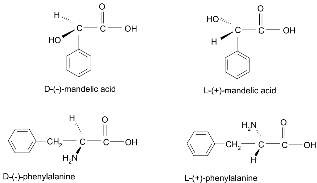
Figure1: Structure of ( \pm )-mandelic acid and ( \pm )-phenylalanine
