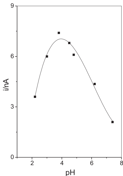
Figure 2. Effect of pH on the biosensor response. Ascorbic acid: 3.0 \times 10^{-4} mol \text{L}^{-1} , flow rate: 0.5 \text{ mL min}^{-1} .
