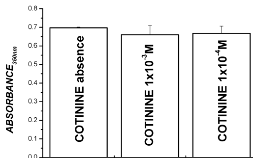
Figure 3. Oxidation of 1 \text{ mmol.L}^{-1} KI by HOCl 0.05 \text{ mmol.L}^{-1} + Tau 0.2 \text{ mmol.L}^{-1} in the presence and absence of cotinine, 1 \text{ mmol.L}^{-1} or 0.1 \text{ mmol.L}^{-1} , followed at 350 nm. TauCl and cotinine were incubated for one minute before KI was added. PBS-D, pH 7.4, 25^\circ\text{C} .
