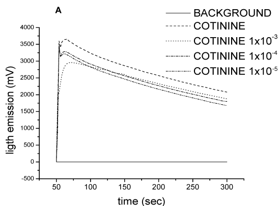
Figure 4. HRP ( 3.10^{-8} \text{ mol.L}^{-1} ) kinetics in presence of \text{H}_2\text{O}_2 ( 1.10^{-5} \text{ mol.L}^{-1} ), and luminol ( 1.10^{-5} \text{ mol.L}^{-1} ); with or without various cotinine molar concentrations; n=3 . PBS-D buffer, pH 7.4; 25^\circ\text{C} . 4A) Light emission kinetics; background is without hydrogen peroxide. 4B) Areas under light emission curves; p \leq 0.05 compared to kinetics without cotinine.
