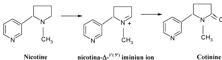
Scheme 1. Nicotine transformation into cotinine by cytochrome P450 [8].
