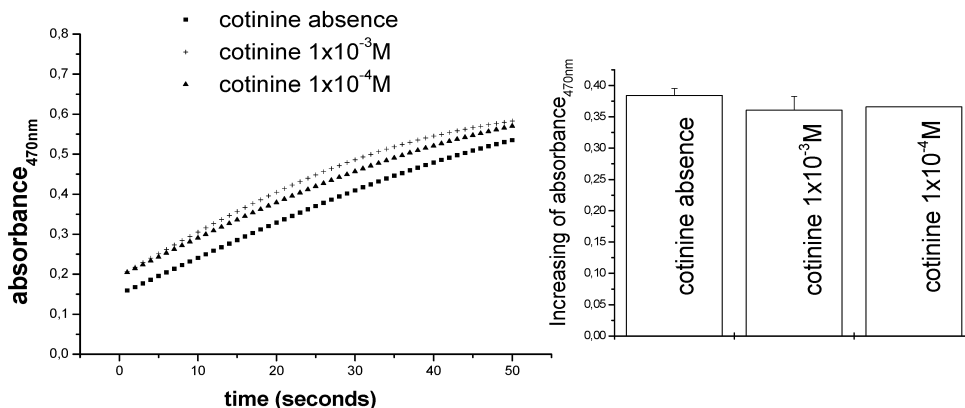
Figure 5. Guaiacol kinetic of oxidation by system HRP 7 nmol.L -1 ; guaiacol 1mmol.L -1 and H 2 O 2 0.1 mmol.L -1 ; λ=470 nm; PBS-D buffer, pH 7.4, 25°C.
