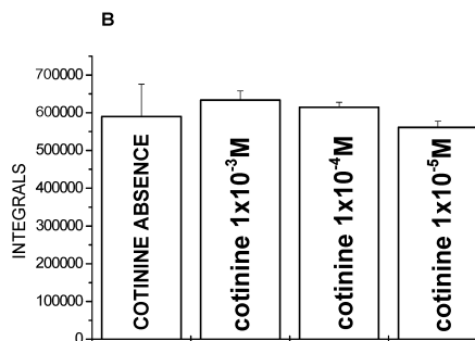
Figure 4. HRP ( 3.10^{-8} \text{ mol.L}^{-1} ) kinetics in presence of \text{H}_2\text{O}_2 ( 1.10^{-5} \text{ mol.L}^{-1} ), and luminol ( 1.10^{-5} \text{ mol.L}^{-1} ); with or without various cotinine molar concentrations; n=3 . PBS-D buffer, pH 7.4; 25^\circ\text{C} . 4A) Light emission kinetics; background is without hydrogen peroxide. 4B) Areas under light emission curves; p \leq 0.05 compared to kinetics without cotinine.
