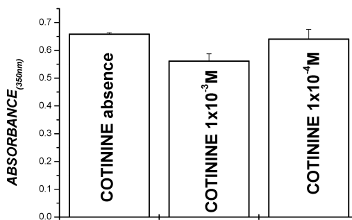
Figure 2. Oxidation of 1 \text{ mmol.L}^{-1} KI by 0.05 \text{ mmol.L}^{-1} HOCl in presence and absence of cotinine, 1 \text{ mmol.L}^{-1} or 0.1 \text{ mmol.L}^{-1} , followed on 350 nm. HOCl and cotinine were incubated for one minute before KI was added. PBS-D, pH 7.4, 25^\circ\text{C} .
