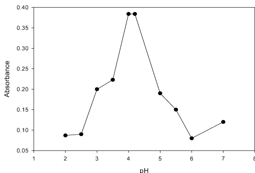
Figure 3. Effect of pH on color intensity for cefotaxime ( 2 \mu\text{g mL}^{-1} ).
