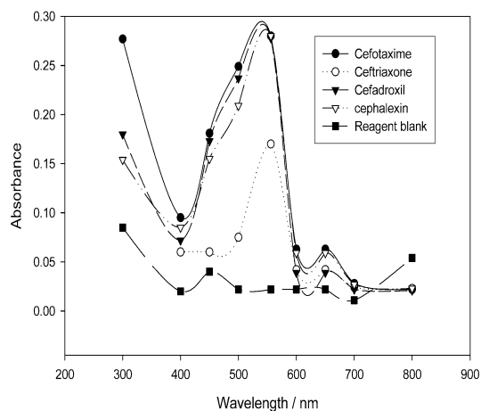
Figure 2. Absorption spectra of colored species of variamine blue with cefotaxime, ceftriaxone, cefadroxil and cephalixin against reagent blank: c (variamine blue) = 0.05%, c (cephalosporins) = 2\ \mu\text{g mL}^{-1} .
