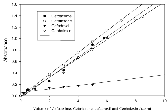
Figure 4. Calibration graphs of cefotaxime, ceftriaxone, cefadroxil and cephalixin: c (cefotaxime) = 0.5 - 5.8 \mu\text{g mL}^{-1} , c (ceftriaxone) = 0.2 - 7.0 \mu\text{g mL}^{-1} , c (cefadroxil) = 0.2 - 5.0 \mu\text{g mL}^{-1} , c (cephalexin) = 0.5 - 8.5 \mu\text{g mL}^{-1} .
