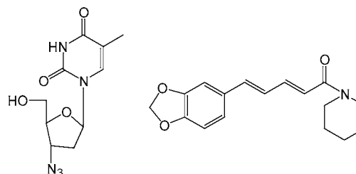
Figure 1. The chemical structure of a : AZT ; b : Piperine.
