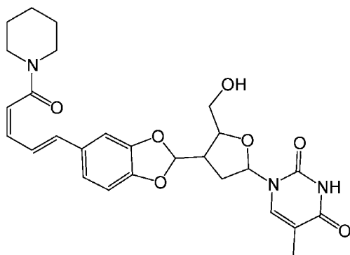
Figure 2. The chemical structure of AHE.
