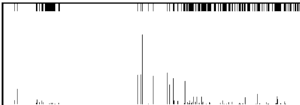
Figure 4. The vibration spectrum of the studied molecules. Normal mode frequencies, varies between 290 and 3520 cm -1 , and infrared band intensities vary between 20 and 360 km mol -1 .
