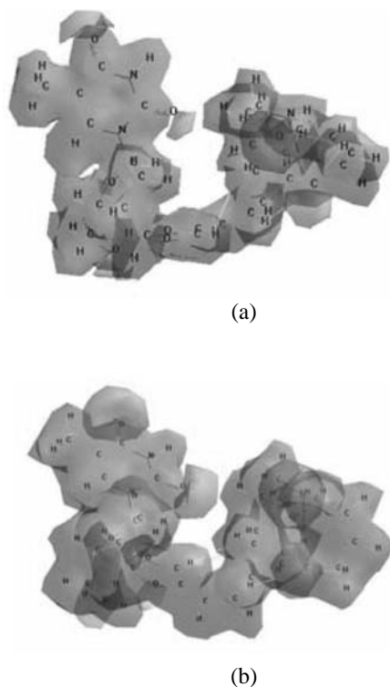
Figure 3. Isosurface of electrostatic potential in the spatial vicinity of AHE. a: AM1 b: DFT.
